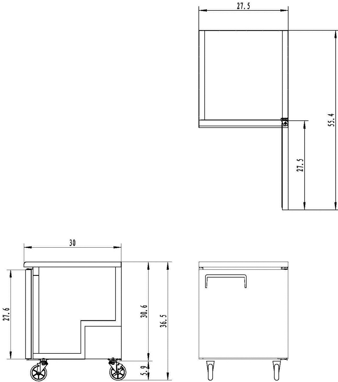
SIDE VIEW
